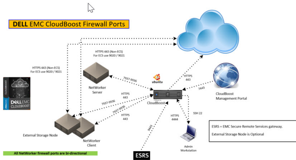
Figure 4 CloudBoost firewall ports
