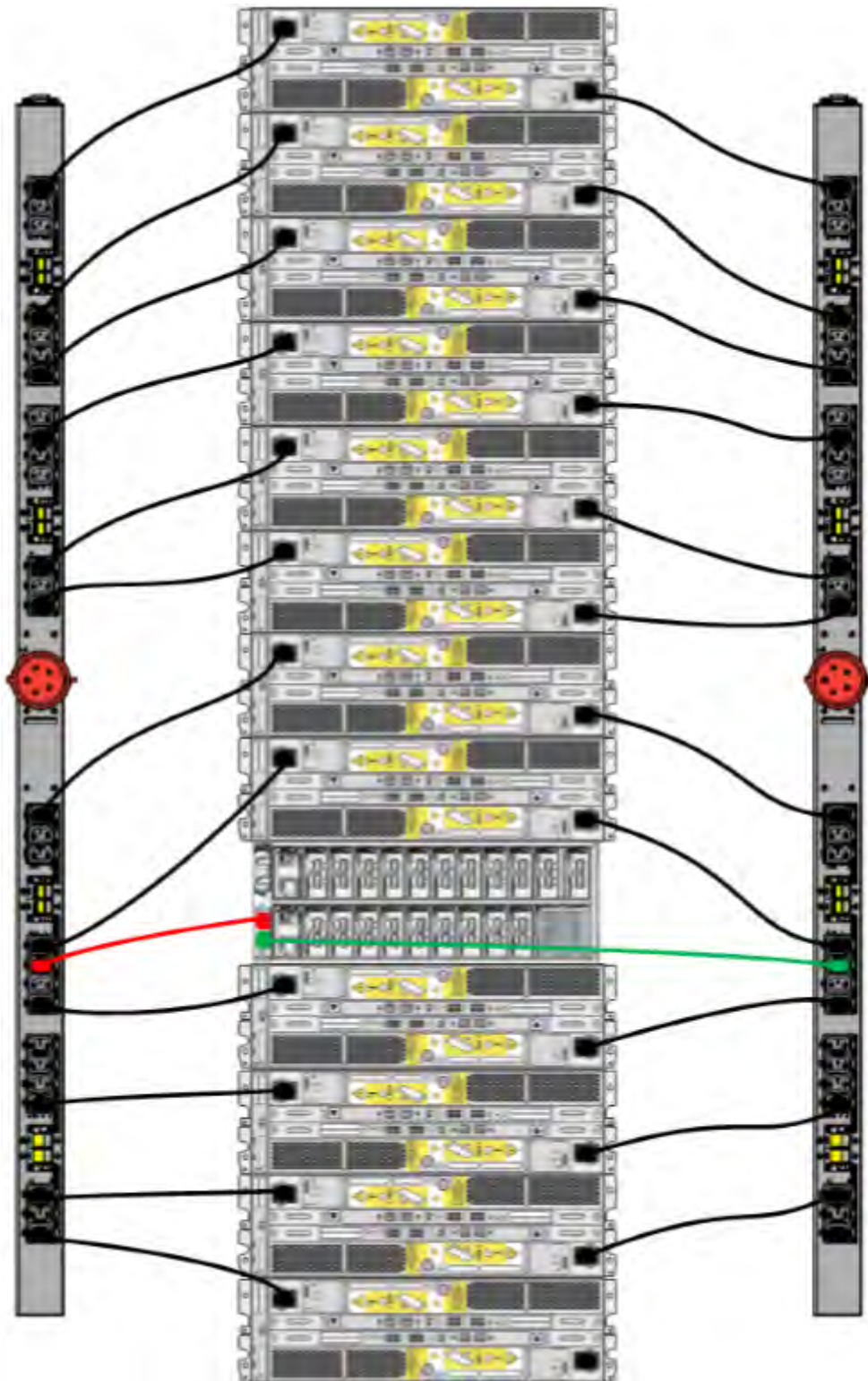
Figure 30. 3-phase wye power connections for DD4200, DD4500, and DD7200
