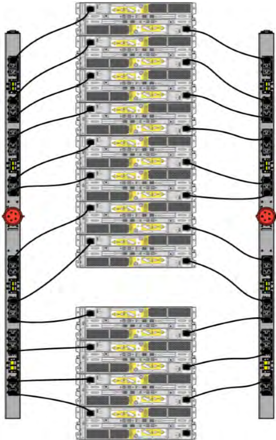
Figure 29. Recommended 3-phase wye power connections for the Expansion Rack
