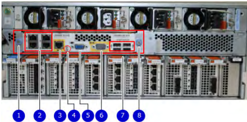
Figure 148. Management module
