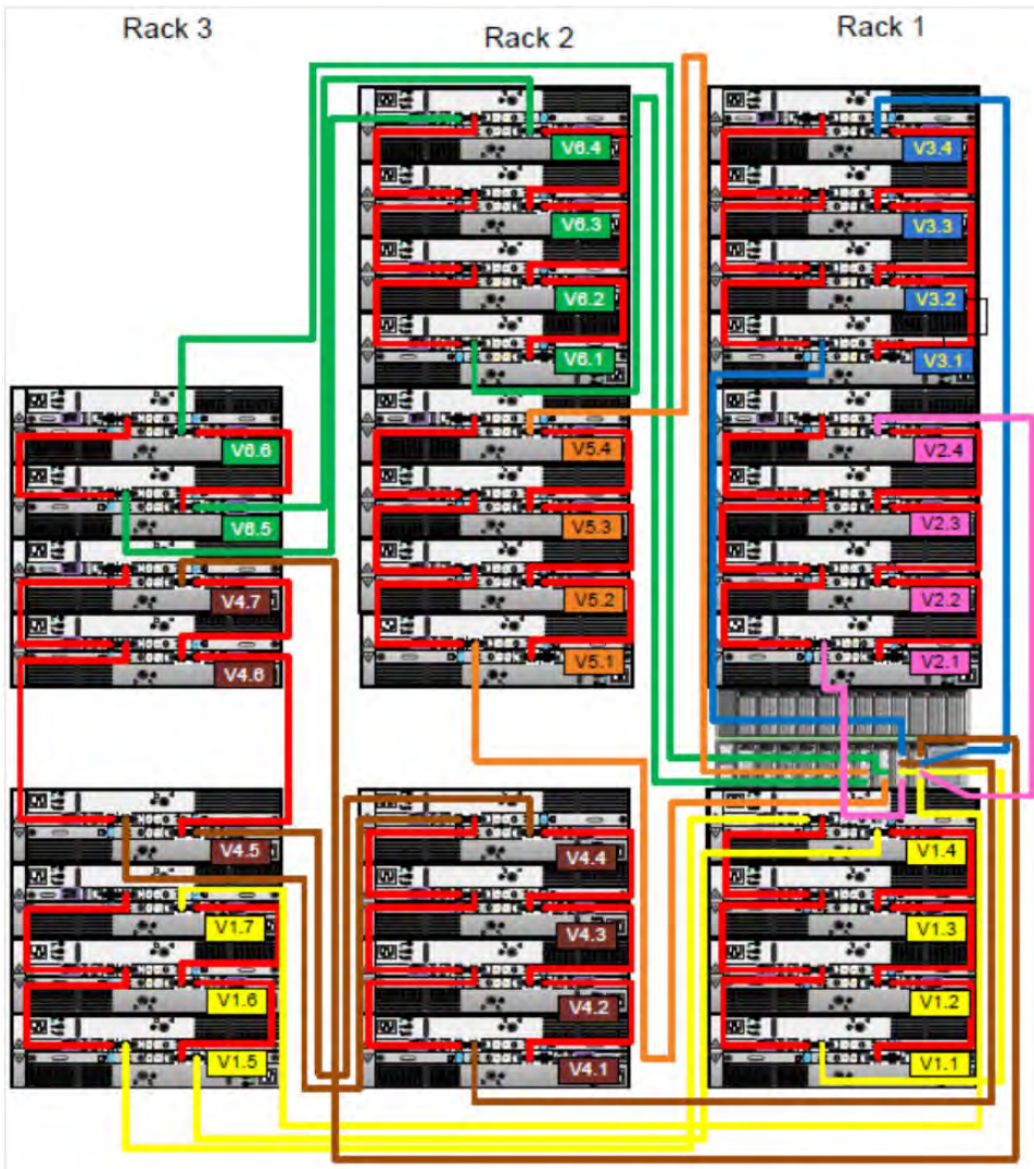
Figure 53. Recommended cabling for DD4500 with extended retention software or DD Cloud Tier
