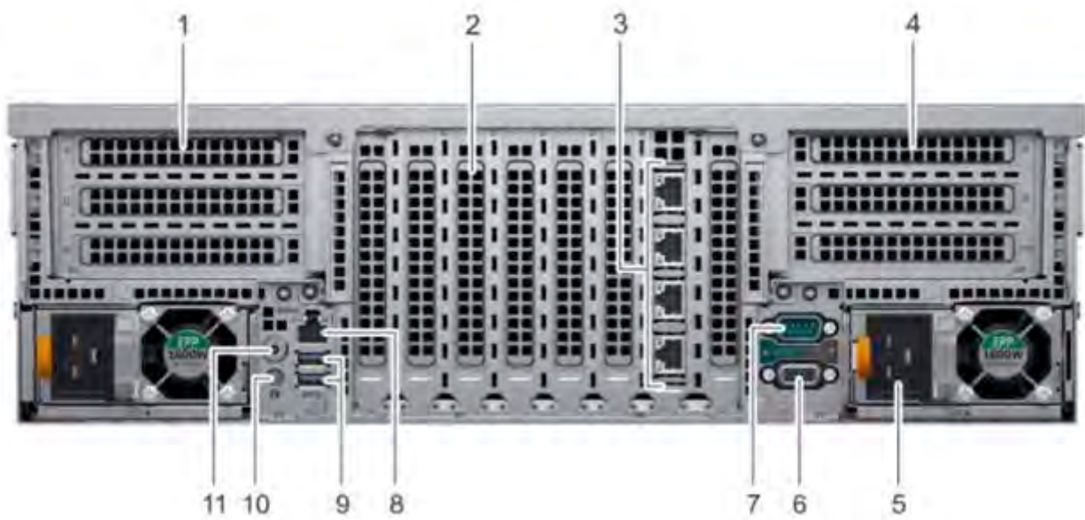
Figure 161. DD9900 rear panel
