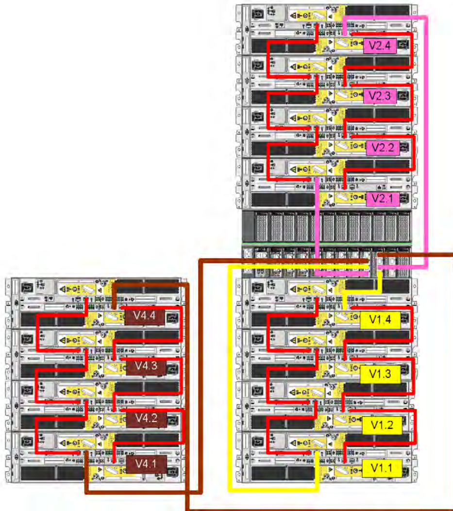
Figure 52. Recommended cabling for DD4500 integrated with Avamar
