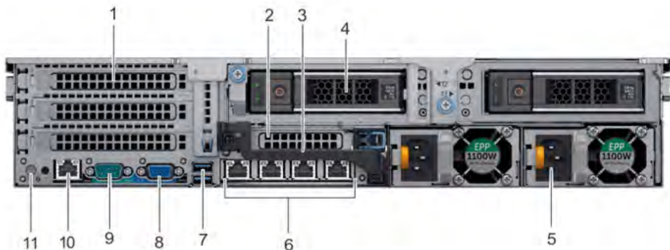
Figure 6. Rear panel
