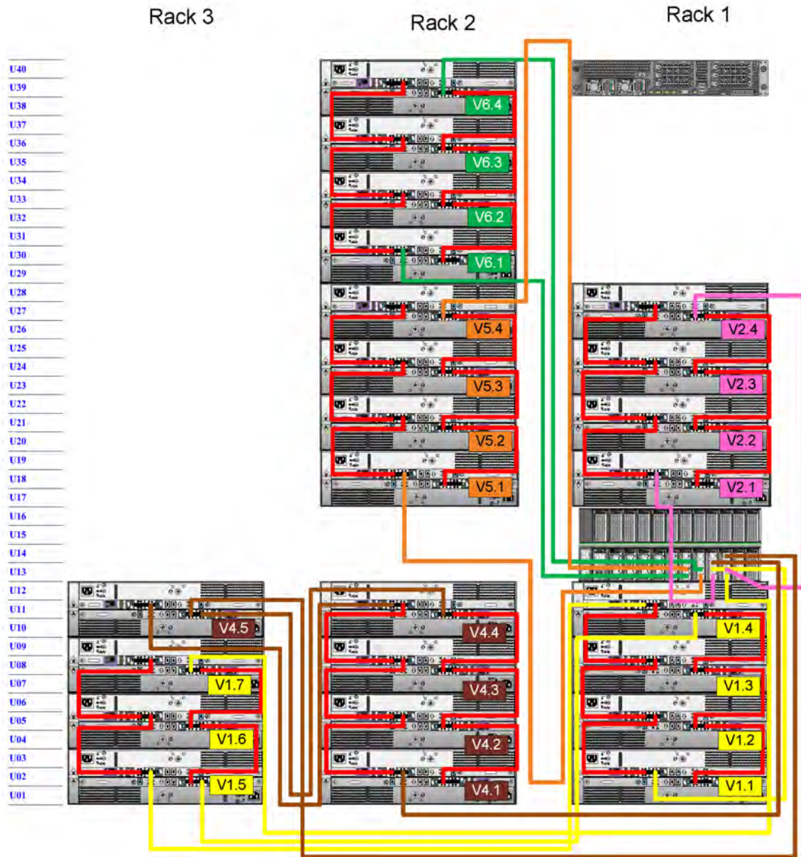
Figure 34. Recommended cabling for DD4200 with extended retention and integrated with Avamar
