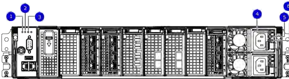
Figure 72. Rear LED indicators
