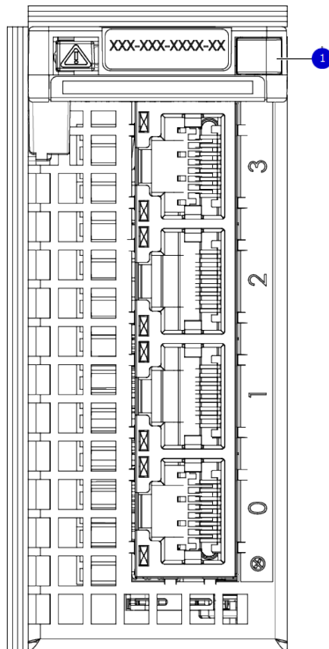
Figure 73. I/O module Power/Service LED location
