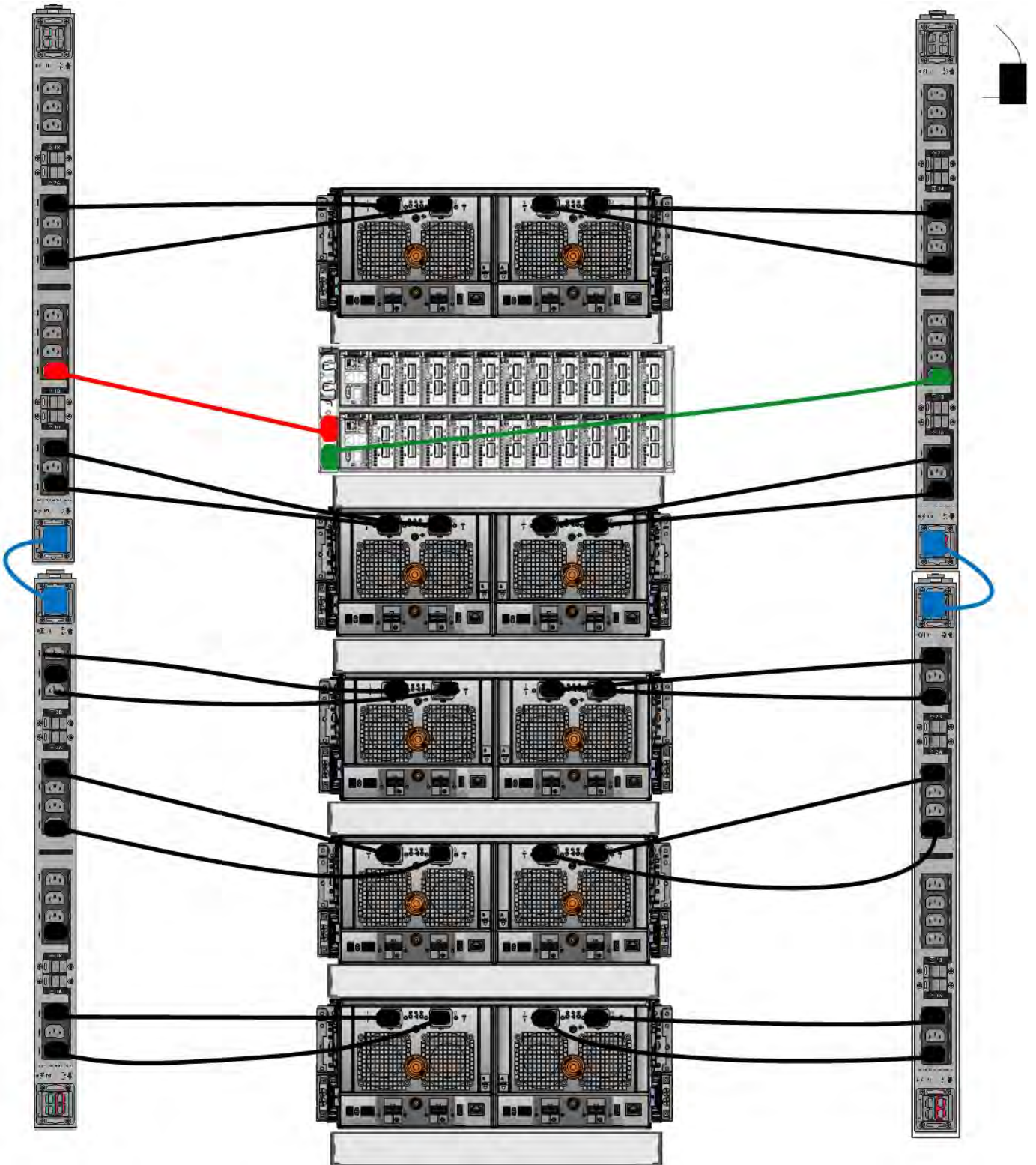
Figure 37. 3-phase delta power connections for DD4200, DD4500, and DD7200 systems
