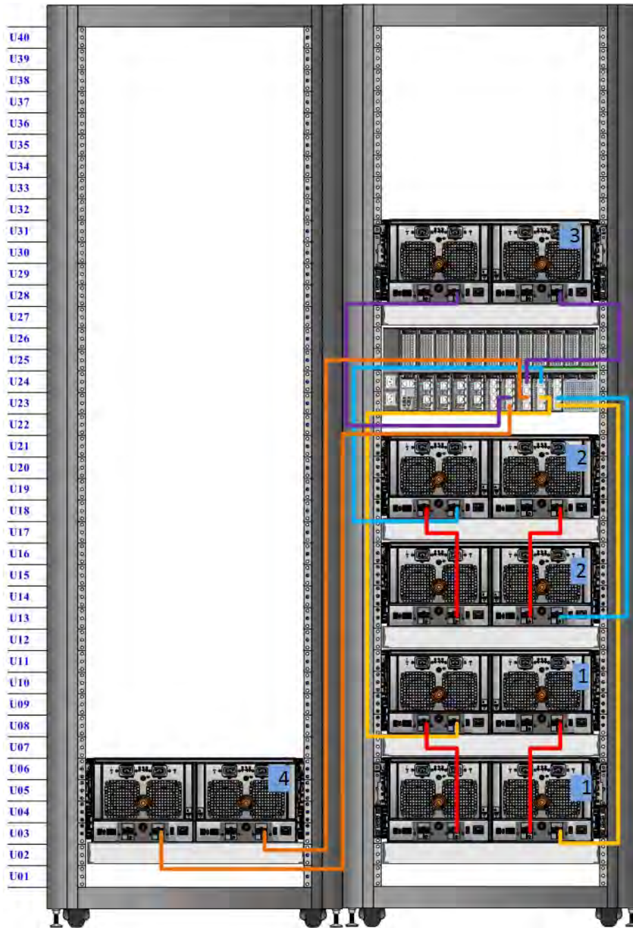
Figure 108. Recommended cabling for DD7200 (4TB drives) with Extended Retention software
