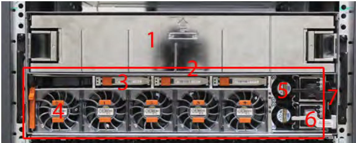
Figure 13. Front panel components
