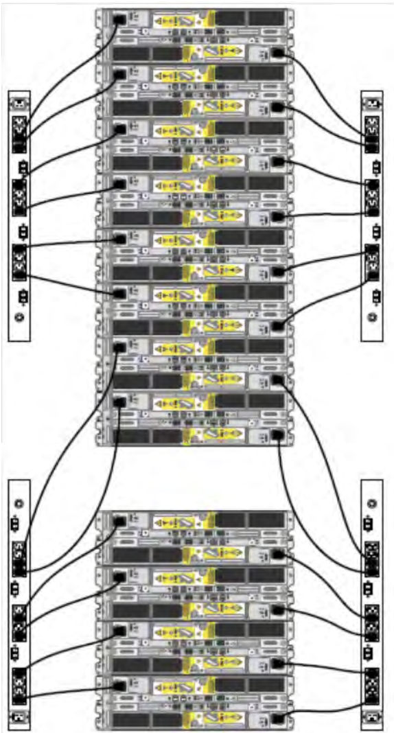
Figure 23. Single phase power connections for the Expansion Rack
