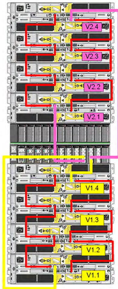
Figure 32. Recommended cabling for DD4200 integrated with Avamar
