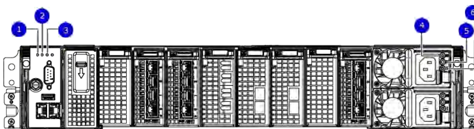
Figure 110. Rear LED indicators
