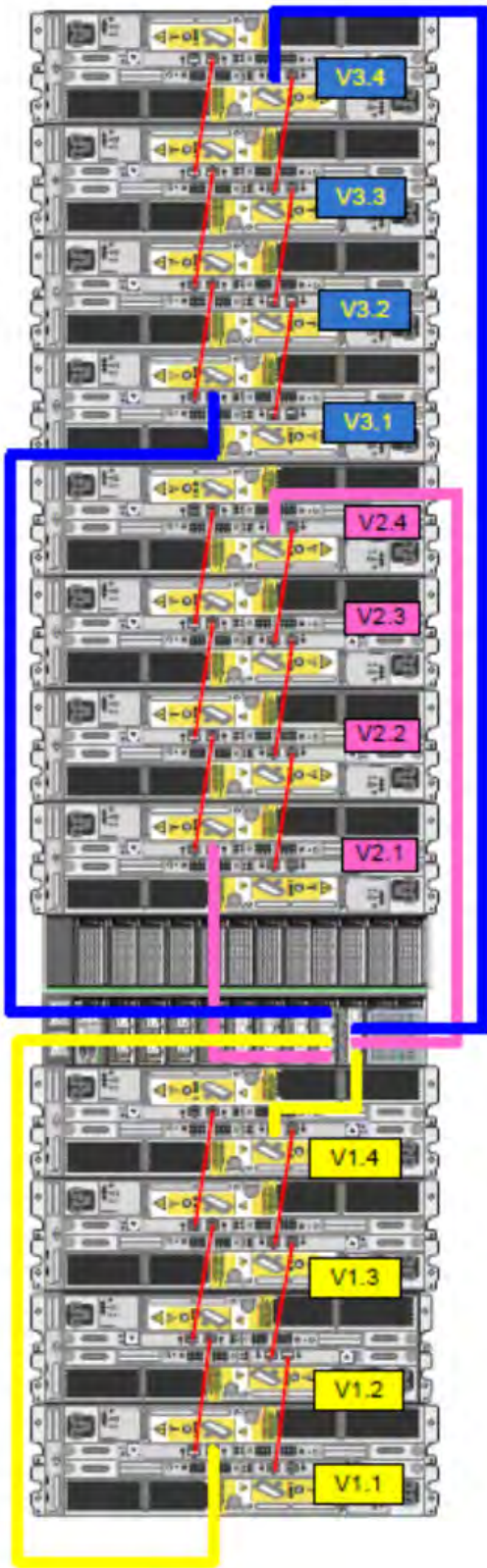
Figure 51. Recommended DD450 cabling
