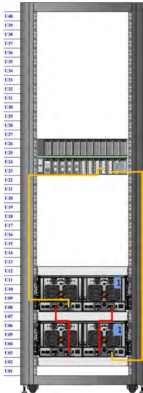
Figure 60. Recommended cabling for DD4500 (3TB drives)
