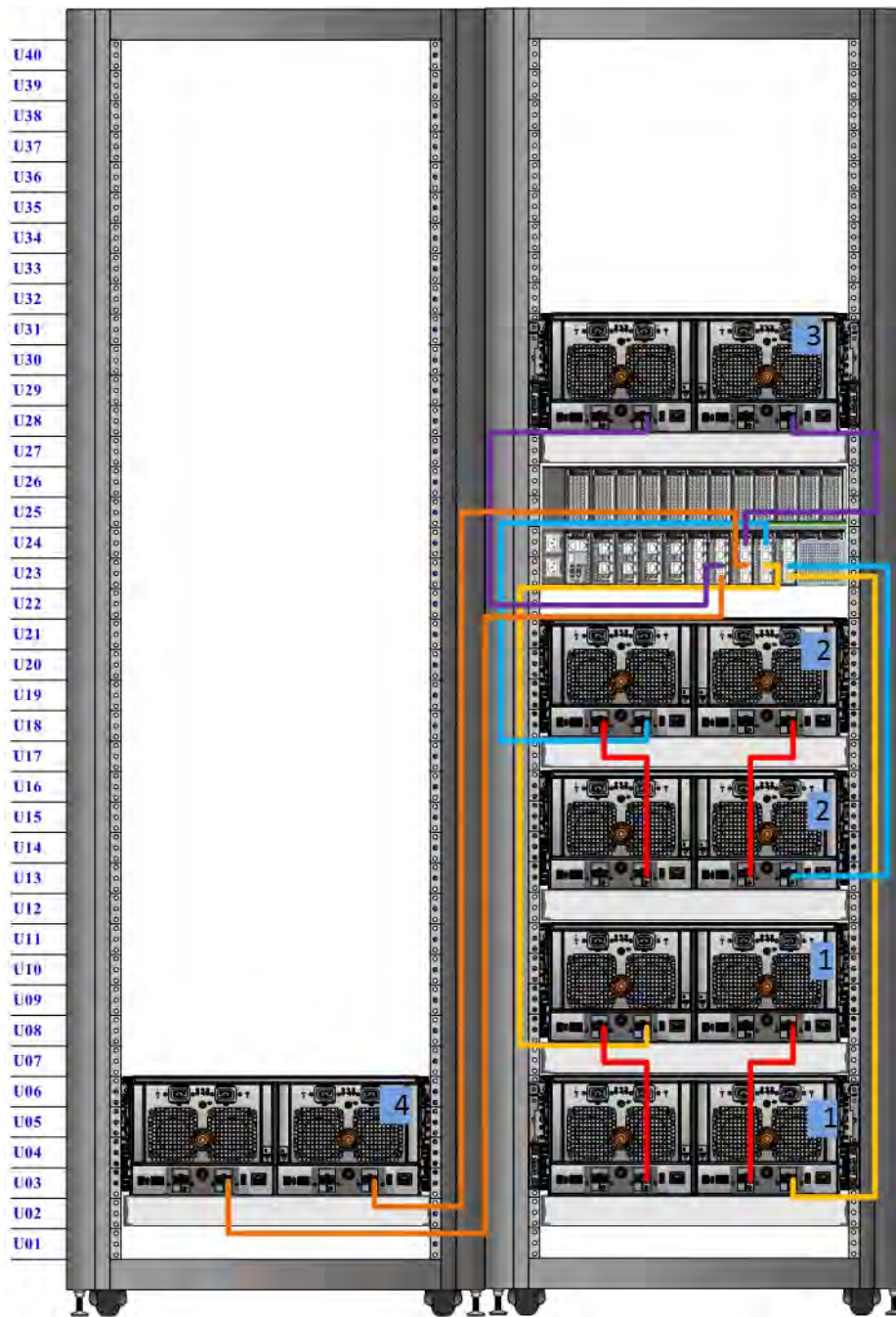
Figure 106. Recommended cabling for DD7200 (3TB drives) with Extended Retention software
