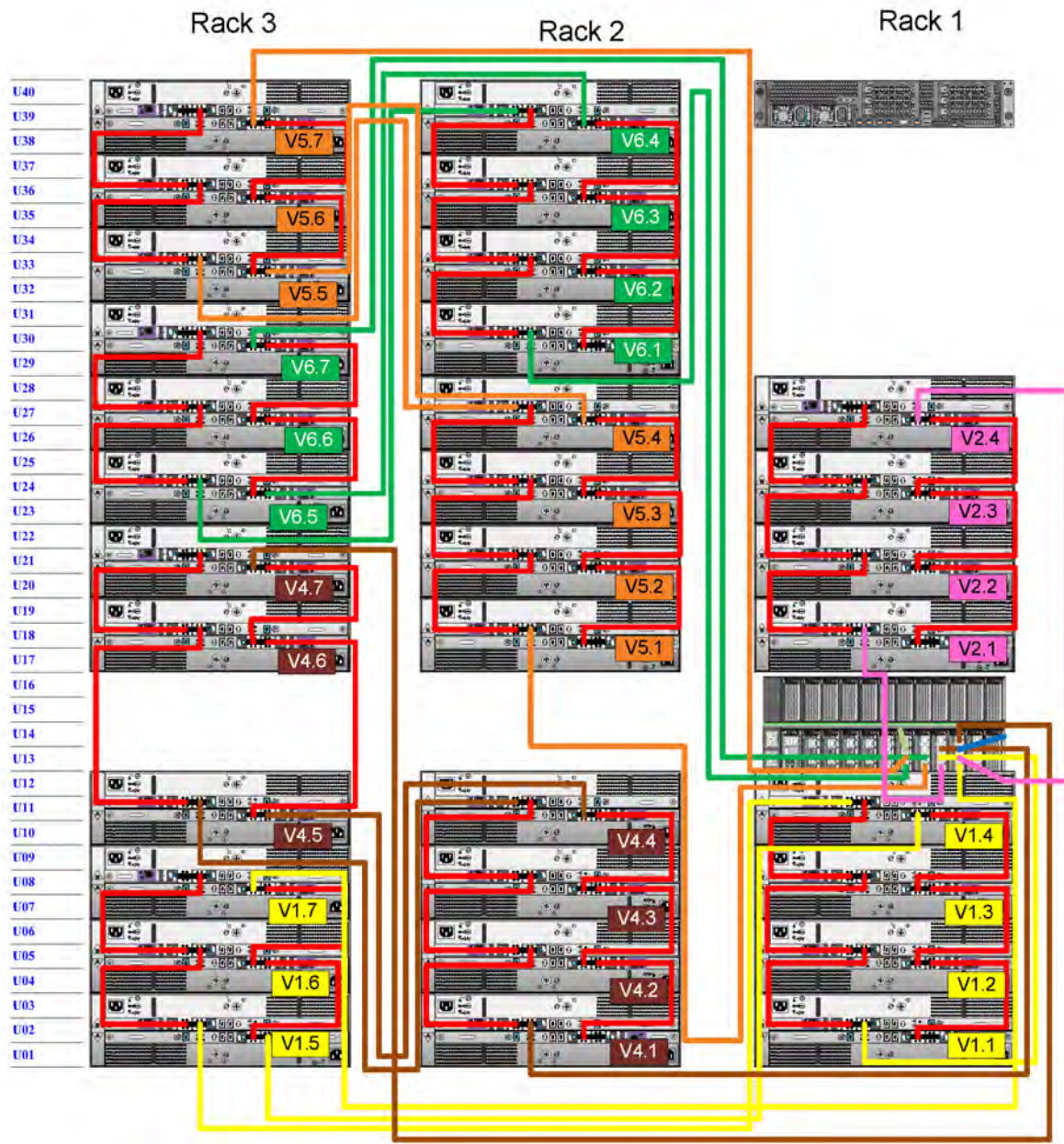
Figure 54. Recommended cabling for DD4500 with extended retention and integrated with Avamar
