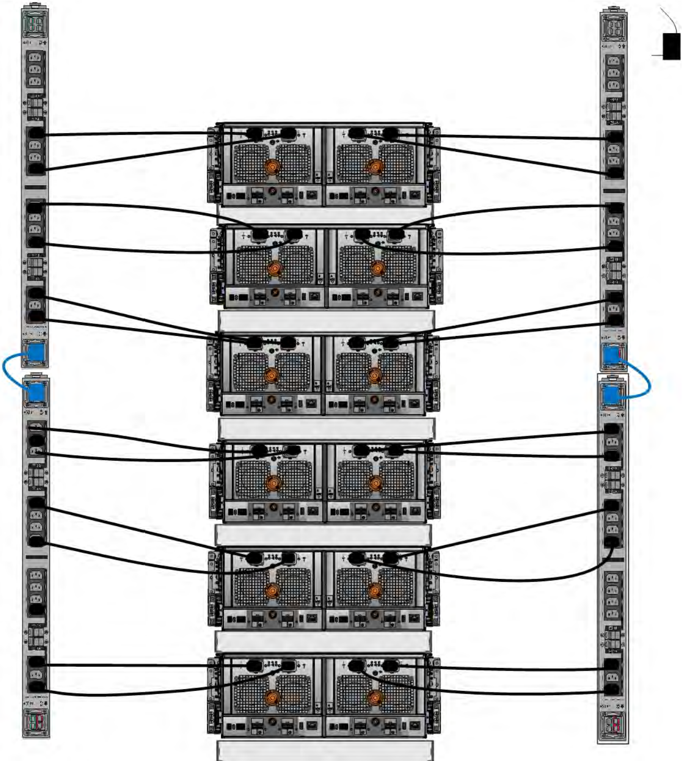
Figure 36. 3-phase delta power connections for DS60 expansion shelves (full-racked)
