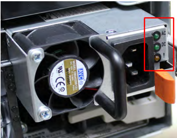
Figure 89. Power supply LEDs
