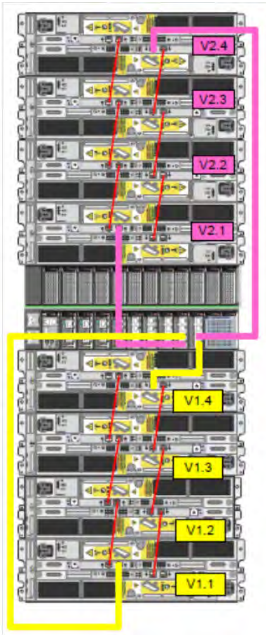
Figure 31. Recommended DD4200 cabling
