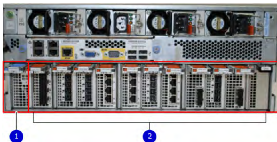
Figure 136. Location of NVRAM and I/O modules
