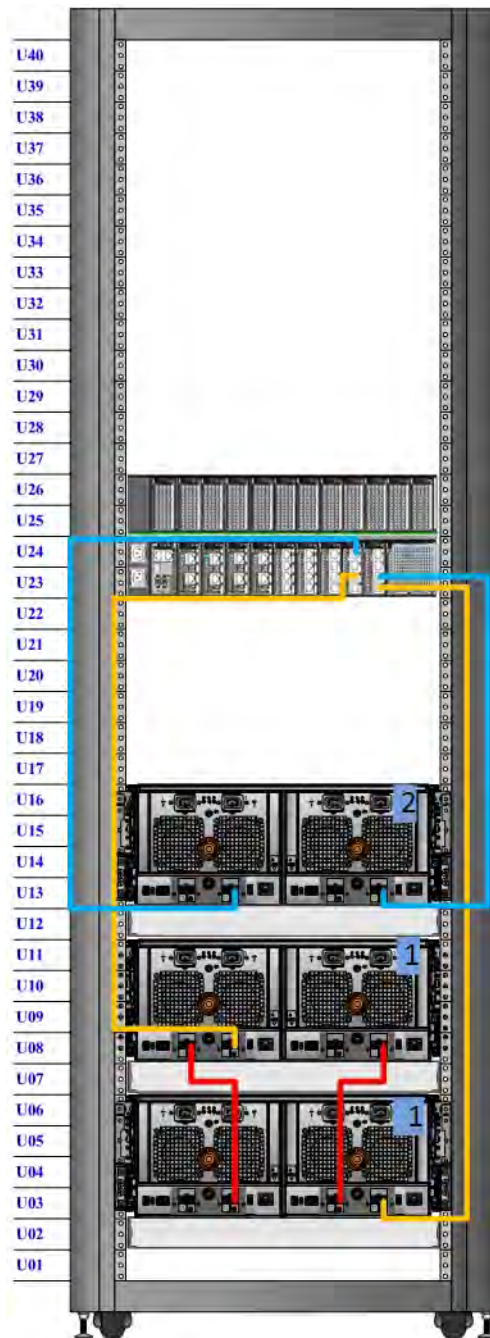
Figure 105. Recommended cabling for DD7200 (4TB drives)
