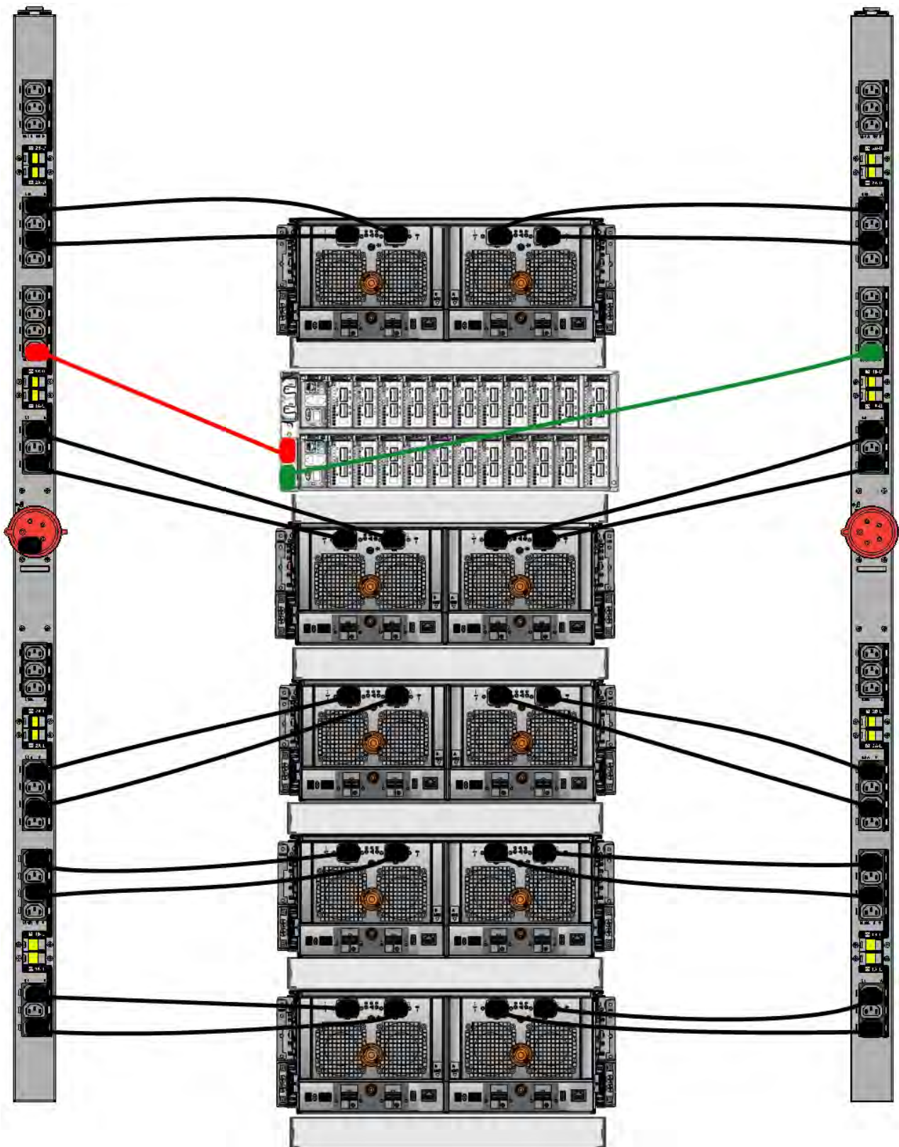
Figure 103. 3-phase wye power connections for DD4200, DD4500, and DD7200 systems
