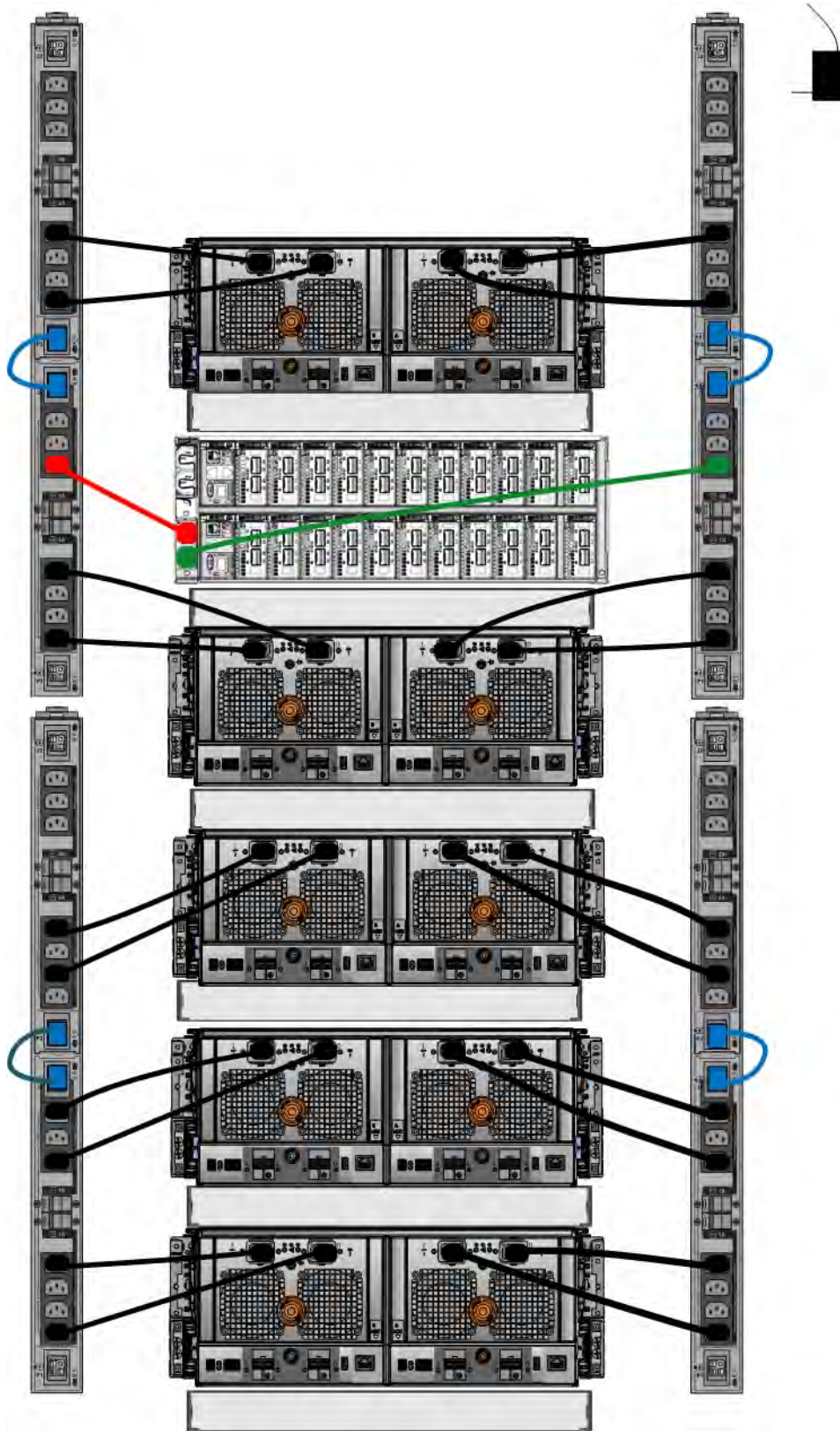
Figure 35. Single phase power connections for DD4200, DD4500, and DD7200 systems
