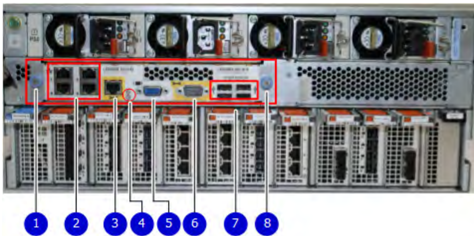
Figure 132. Management module
