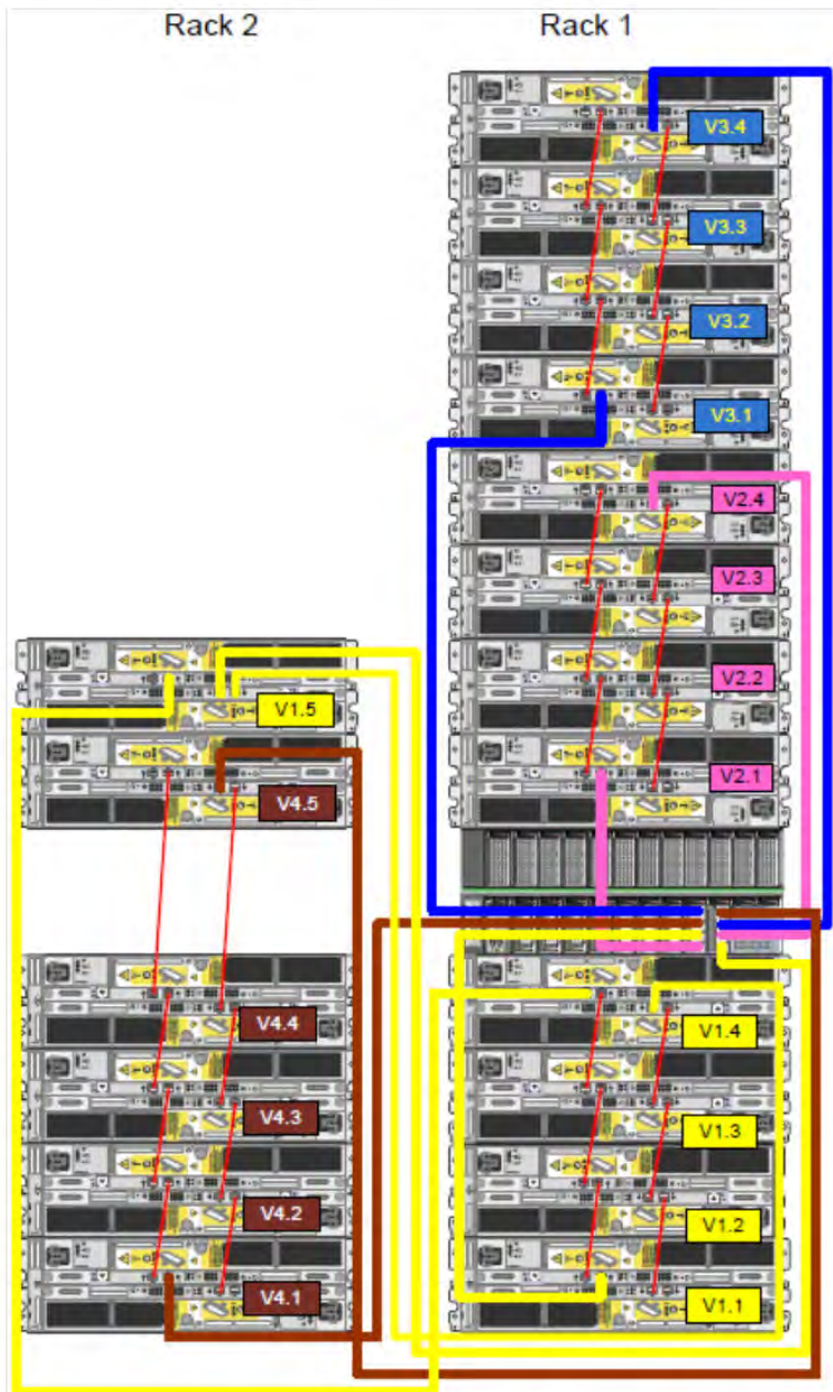
Figure 95. Recommended DD7200 cabling
