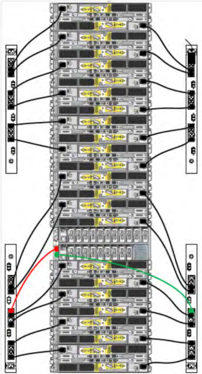
Figure 24. Single phase power connections for the DD4200, DD4500, and DD7200
