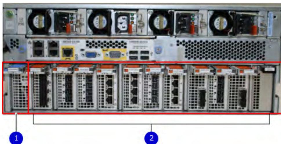
Figure 152. Location of NVRAM and I/O modules
