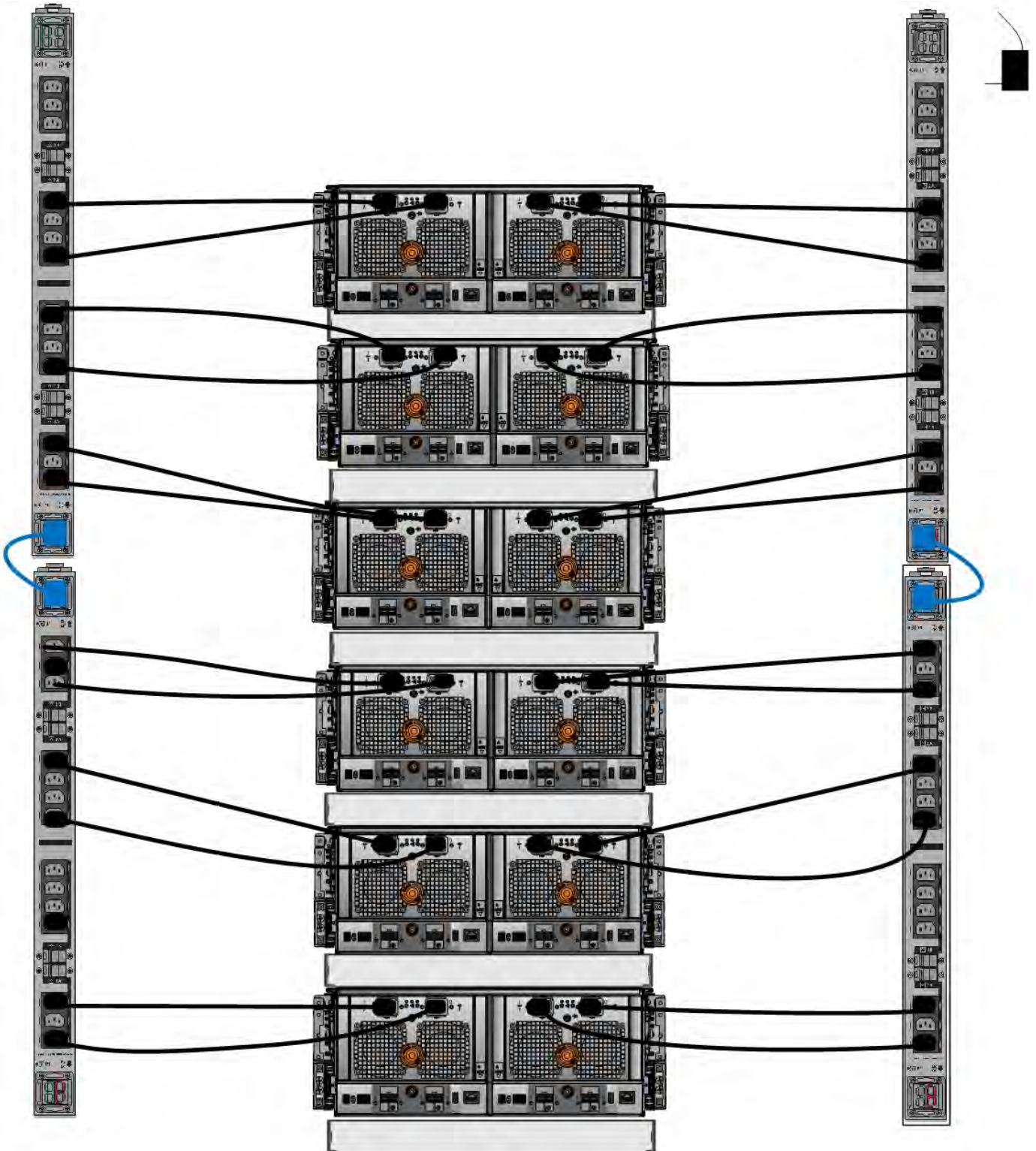
Figure 56. 3-phase delta power connections for DS60 expansion shelves (full-racked)
