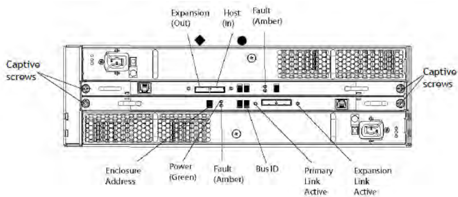
Figure 177. Rear panel overview
