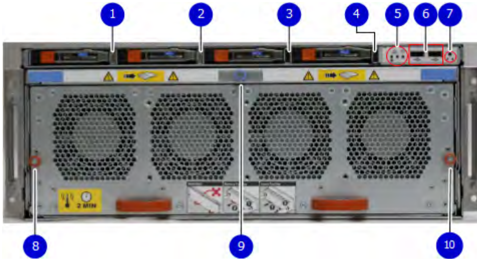
Figure 140. Front panel components
