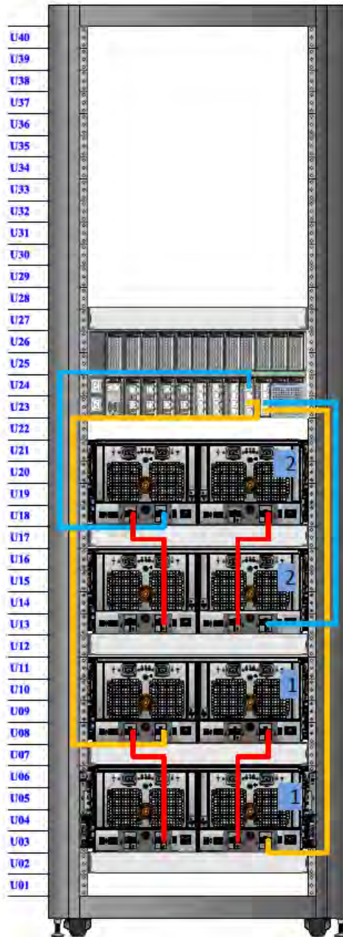
Figure 107. Recommended cabling for DD7200 with DD Cloud Tier
