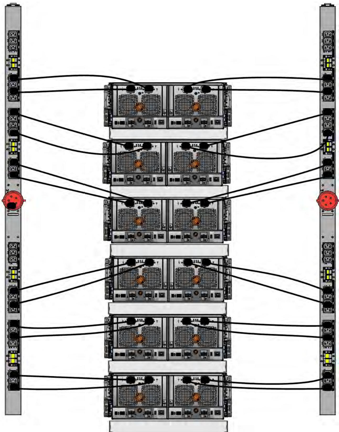
Figure 102. 3-phase wye power connections for DS60 expansion shelves (full-racked)
