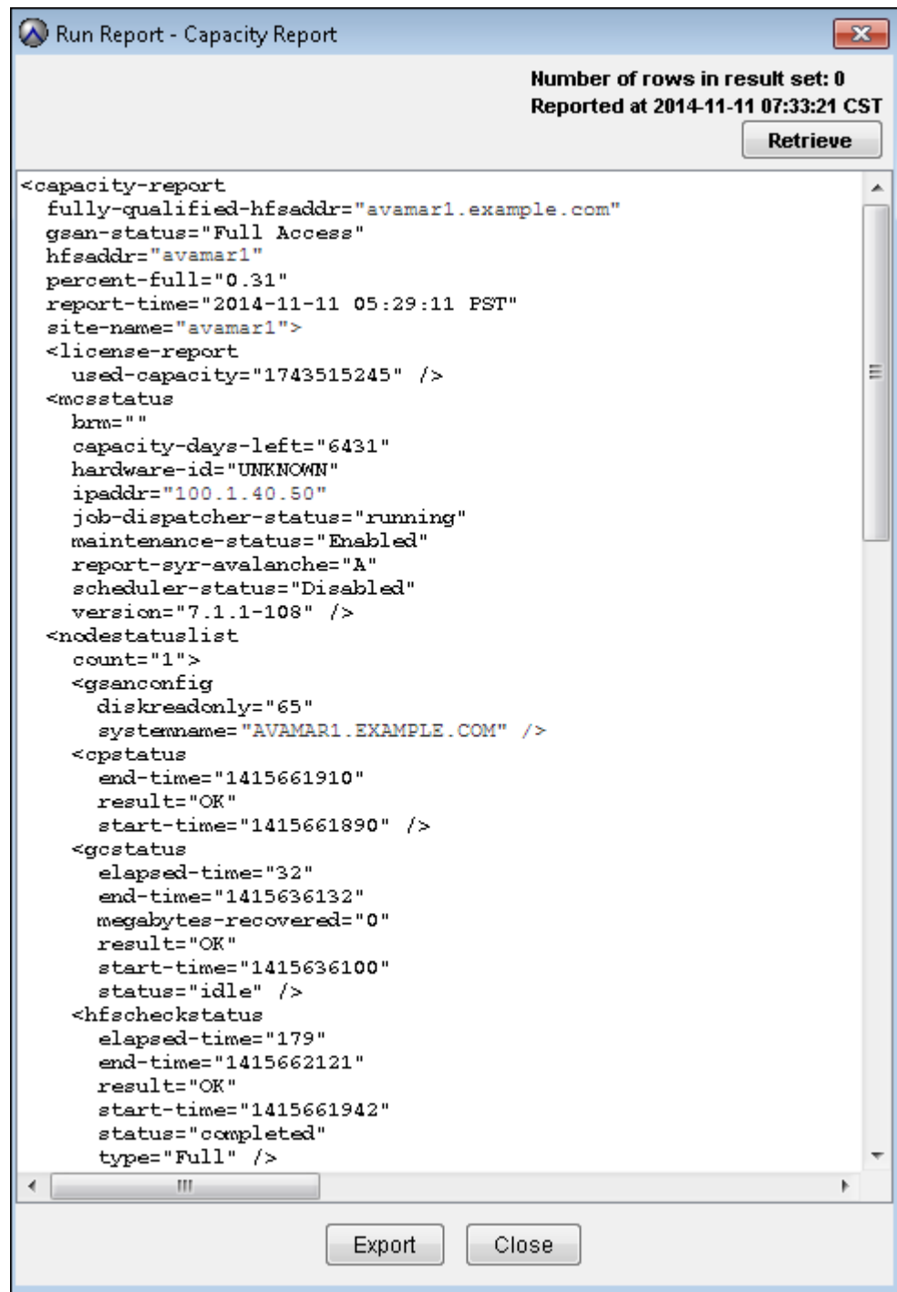
Figure 2 Run Report - Capacity Report dialog box
