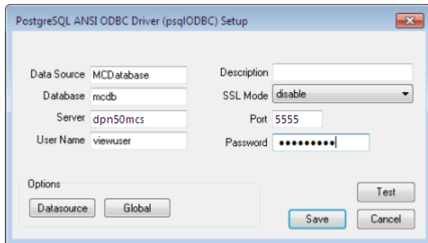
Figure 8 PostgreSQL ODBC Driver (psqlODBC) Setup dialog box
