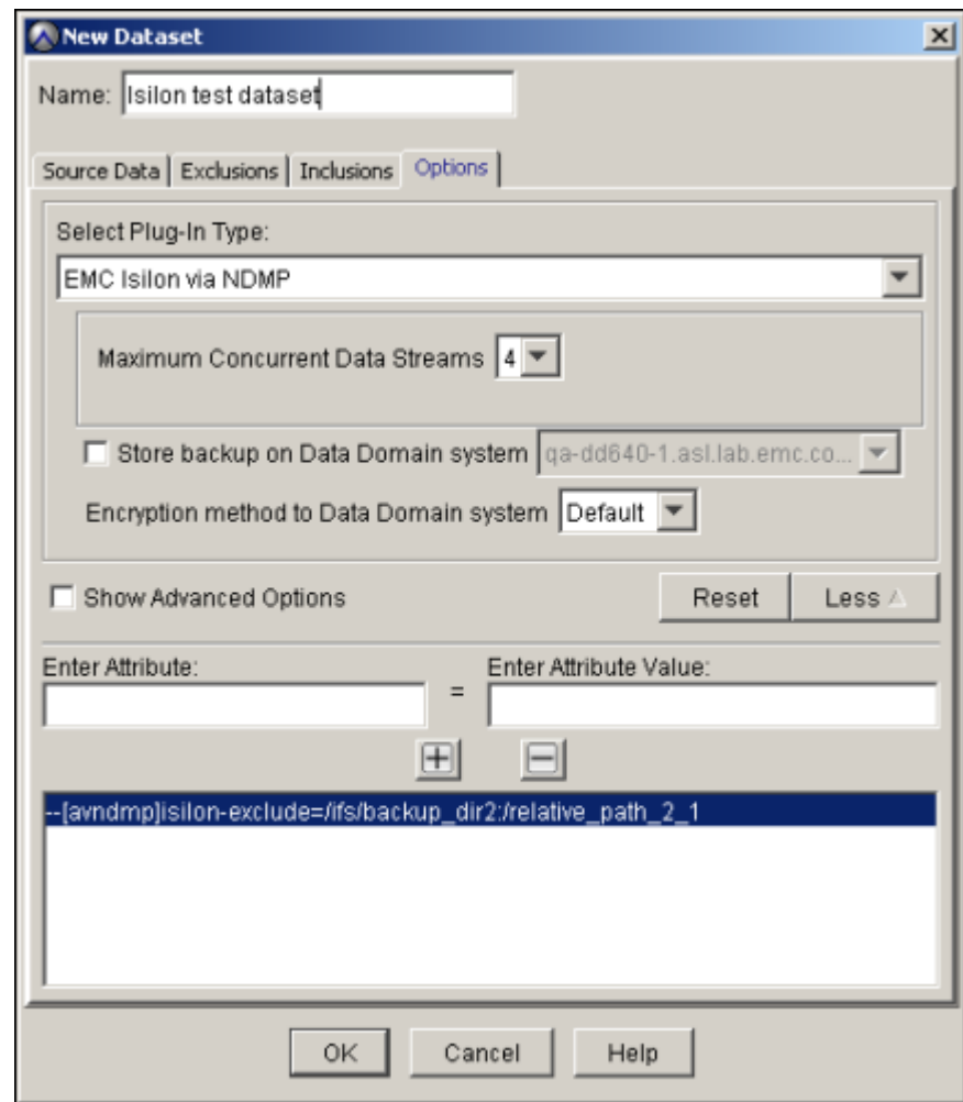
Figure 11 New Dataset window
