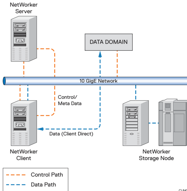
Figure 6 Updated network
