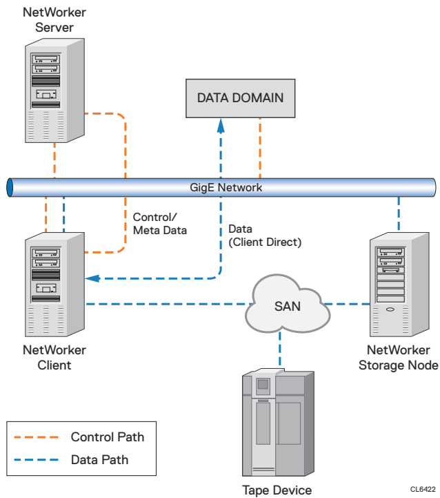
Figure 8 Dedicated SAN
