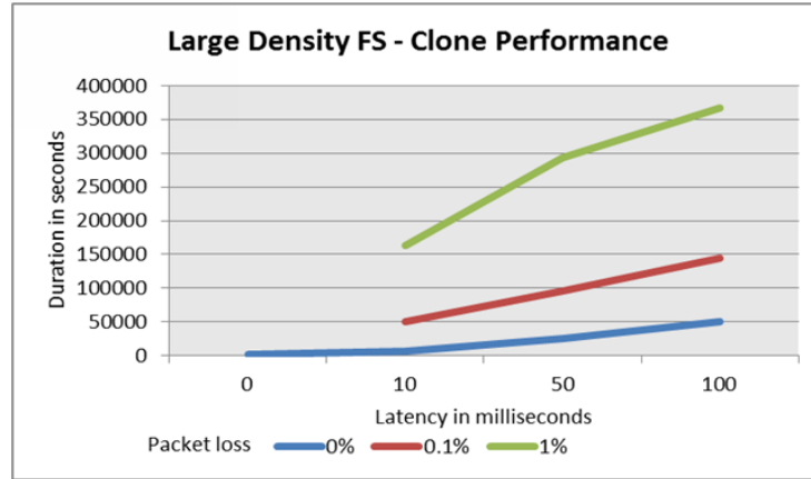
Figure 20 Large Density FS Clone Performance - WAN between NetWorker Clients and Data Domain
