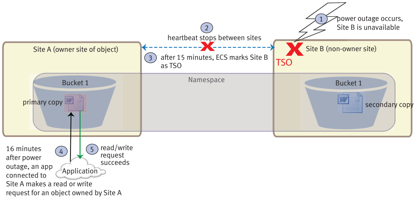
Figure 38 Read/write request succeeds during TSO when data is accessed from owner site and non-owner site is unavailable
