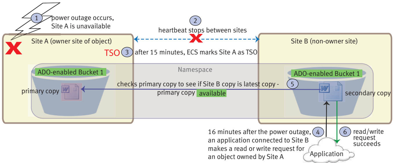
Figure 39 Read/write request succeeds during TSO when ADO-enabled data is accessed from non-owner site and owner site is unavailable
