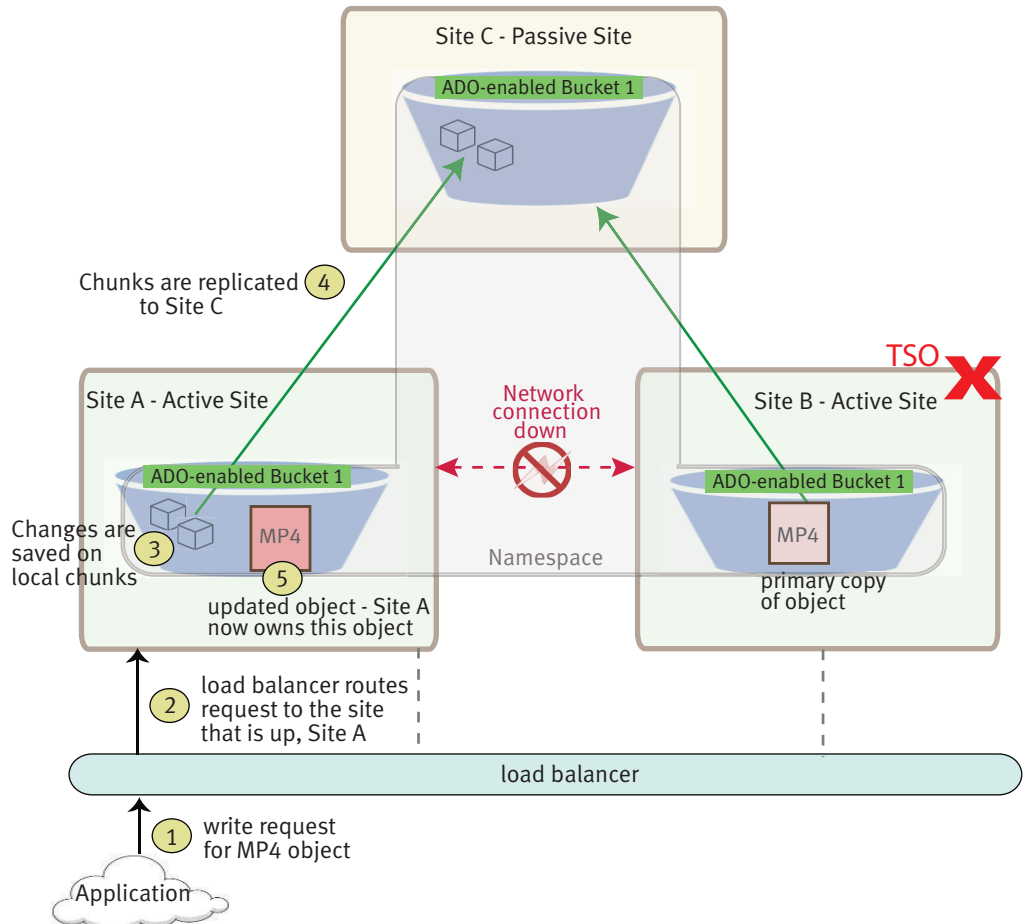
Figure 43 TSO for passive replication
