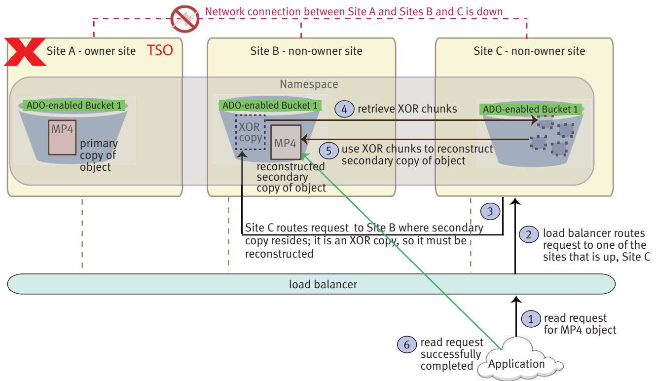
Figure 41 Read request workflow example during a TSO in a three-site federation
