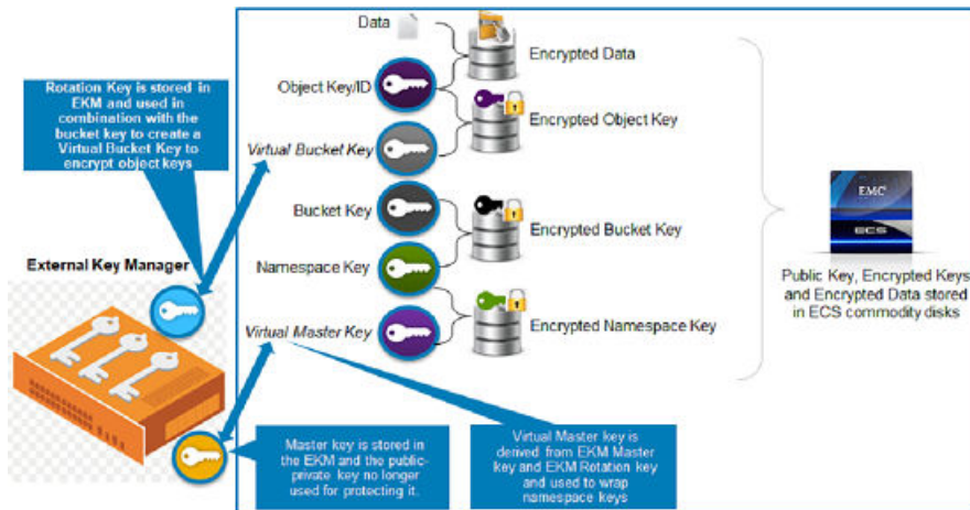
Figure 23 External key management
