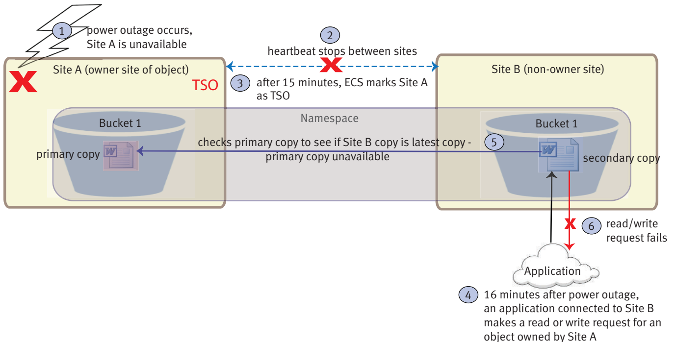
Figure 37 Read/write request fails during TSO when data is accessed from non-owner site and owner site is unavailable
