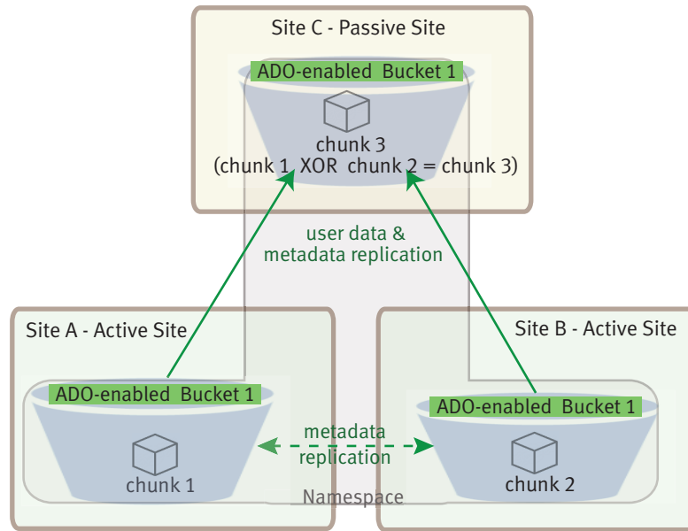
Figure 42 Passive replication in normal state
