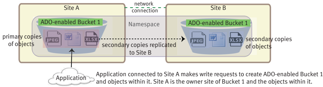
Figure 40 Object ownership example for a write during a TSO in a two-site federation
