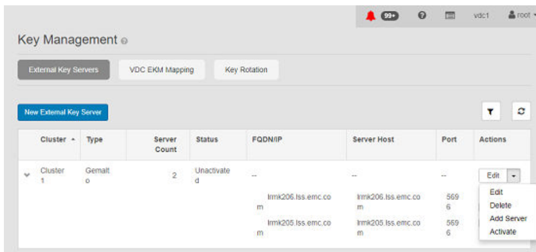
Figure 30 Activate EKM cluster
