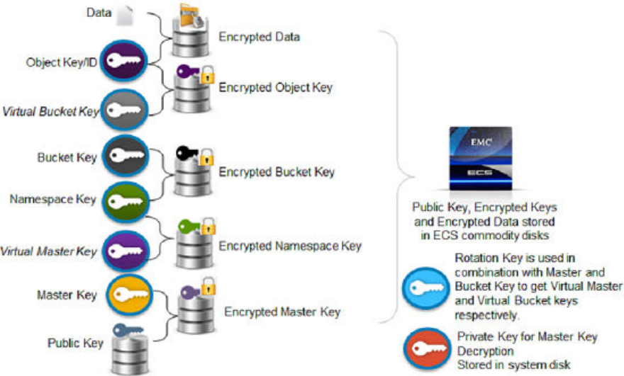
Figure 22 Native key management
