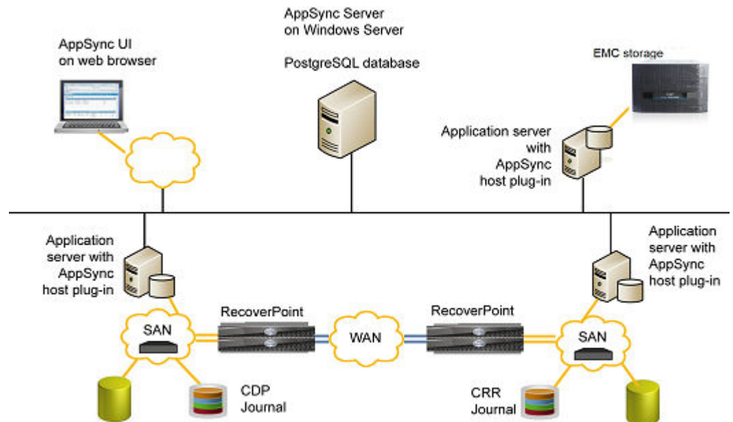
Figure 1 AppSync architecture flow
