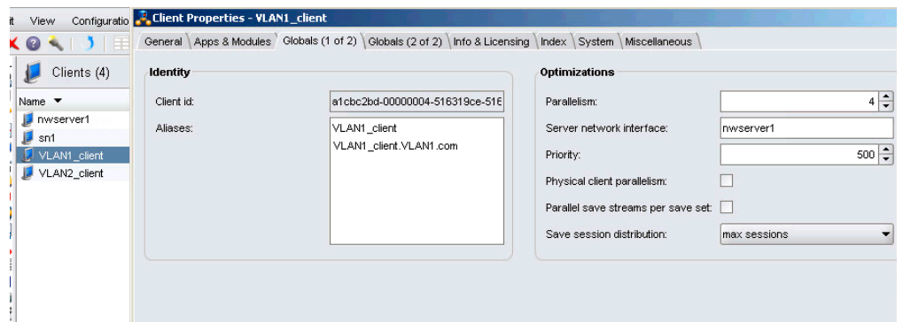
Figure 99 Aliases and Server network interface attributes for VLAN1 clients
