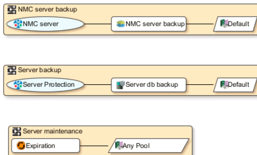
Figure 28 Visual representation of the Server Protection workflows
