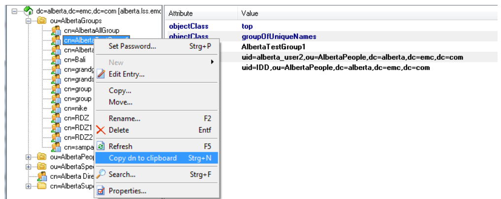
Figure 83 Copying the group DN
