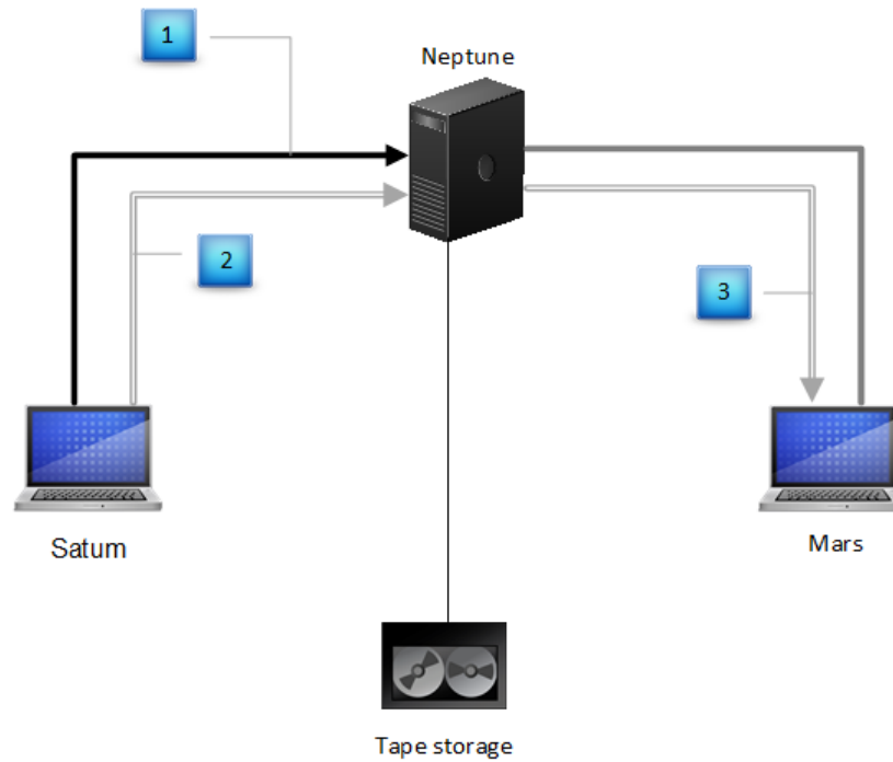
Figure 54 A directed recovery from a remote client
