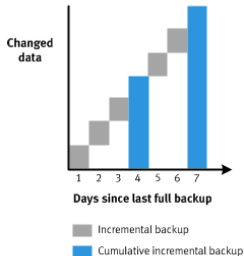
Figure 41 Incremental and cumulative incremental backup levels
