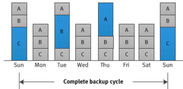
Figure 44 Staggered weekly backup schedule for multiple groups of clients
