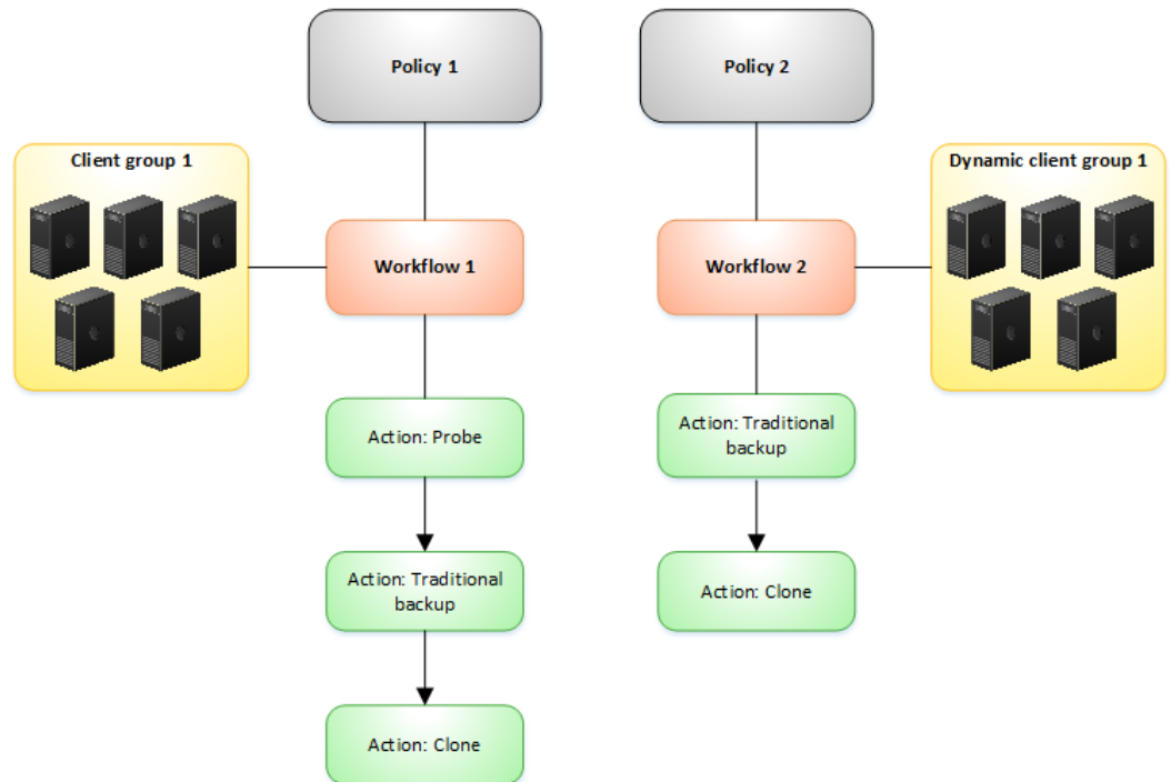
Figure 22 Data protection policy example
