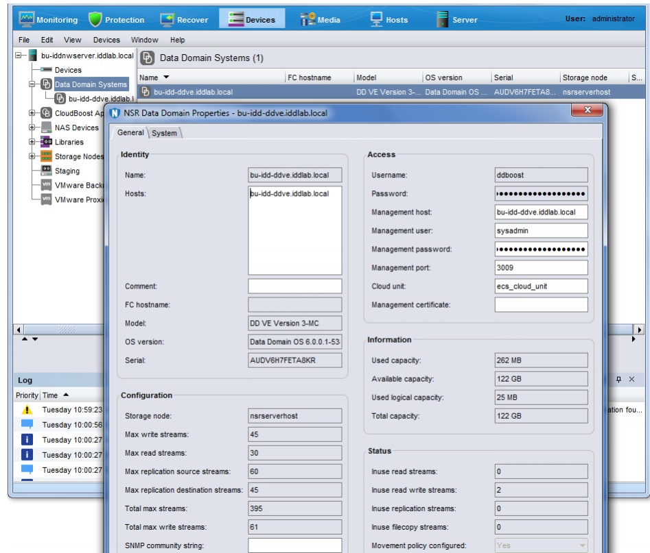
Figure 55 NSR Data Domain Properties
