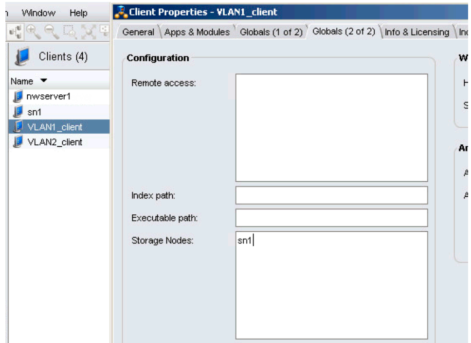
Figure 98 Storage Nodes attribute for clients in VLAN1
