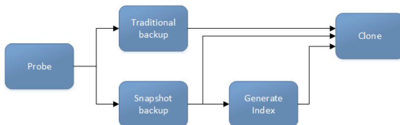
Figure 33 Workflow path from a probe action
