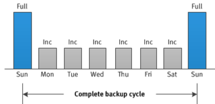
Figure 43 Default weekly backup schedule
