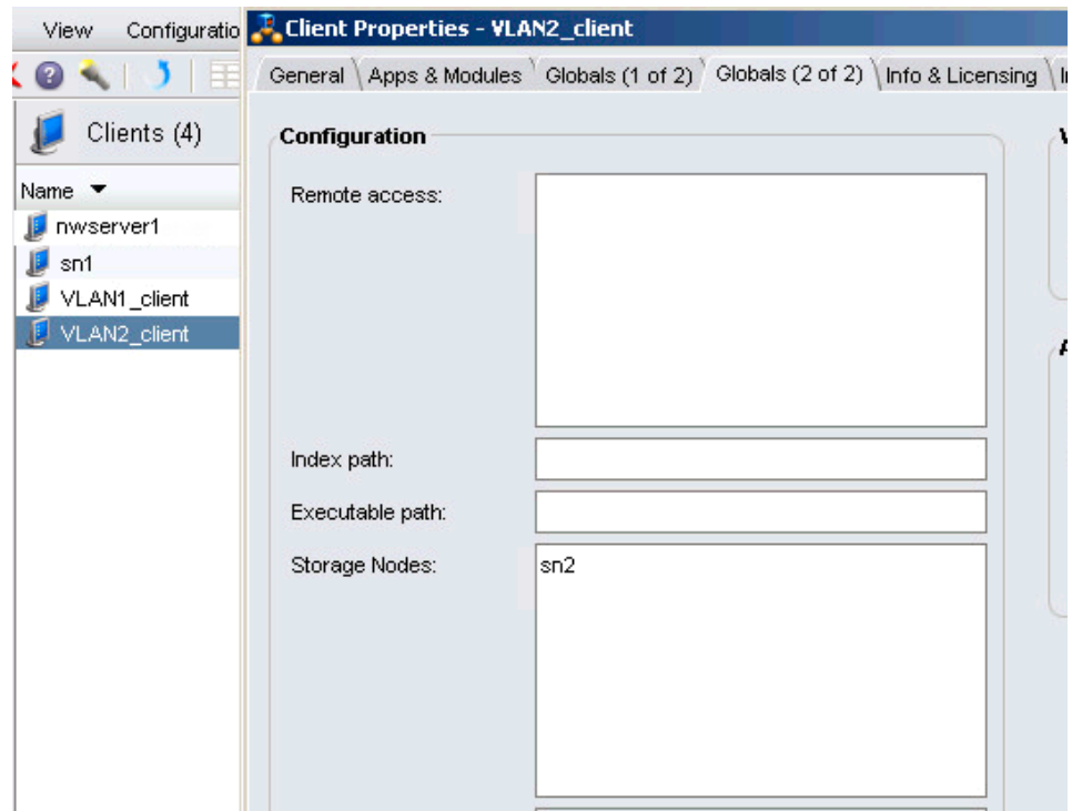
Figure 100 Storage Nodes attribute for clients in VLAN2
