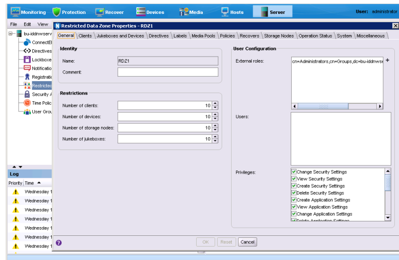
Figure 94 Restricted Datzone User Configuration
