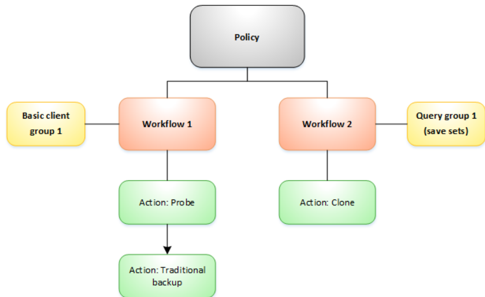
Figure 31 Example of a policy with separate workflows for backup and cloning
