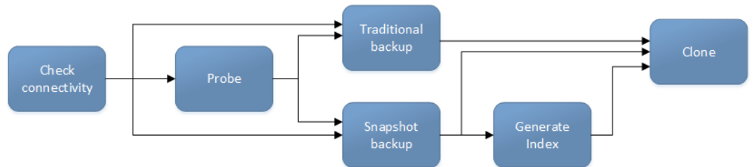
Figure 35 Workflow path from a check connectivity action
