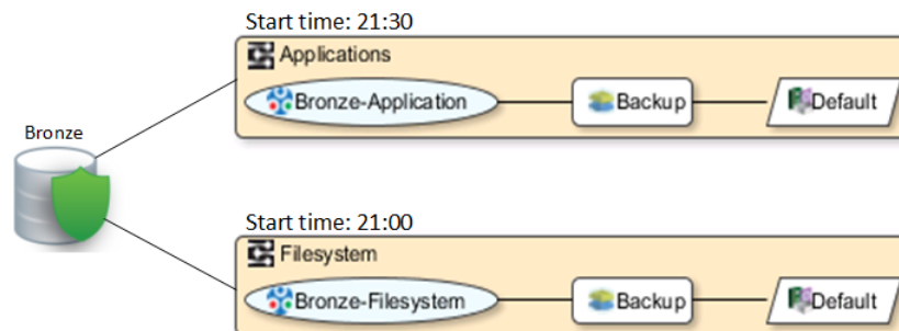
Figure 21 Bronze policy configuration
