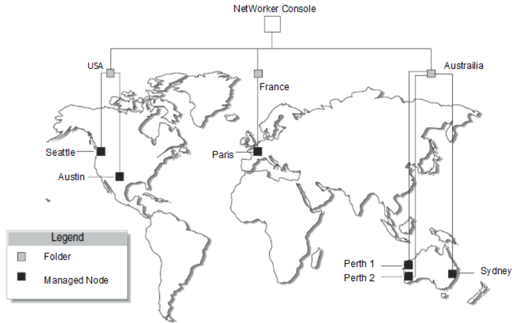
Figure 80 NetWorker servers worldwide
