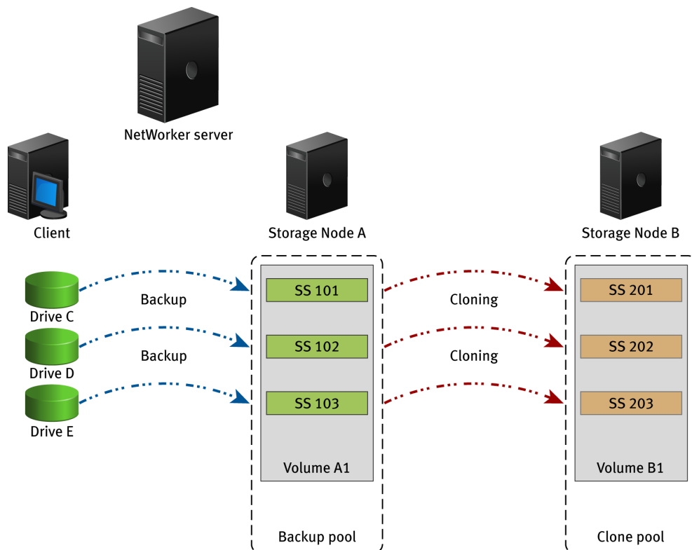
Figure 49 Cloning example
