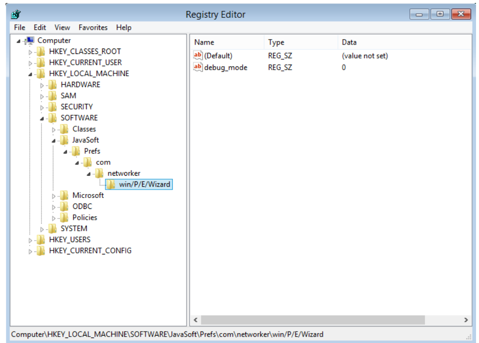
Figure 102 WinPE registry key to troubleshoot recoveries
