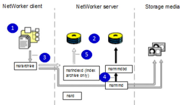
Figure 50 Overview of archive operation
