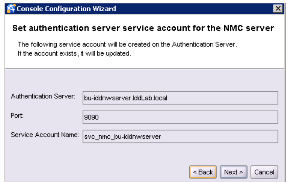
Figure 6 Set authentication server service account for the NMC Server page
