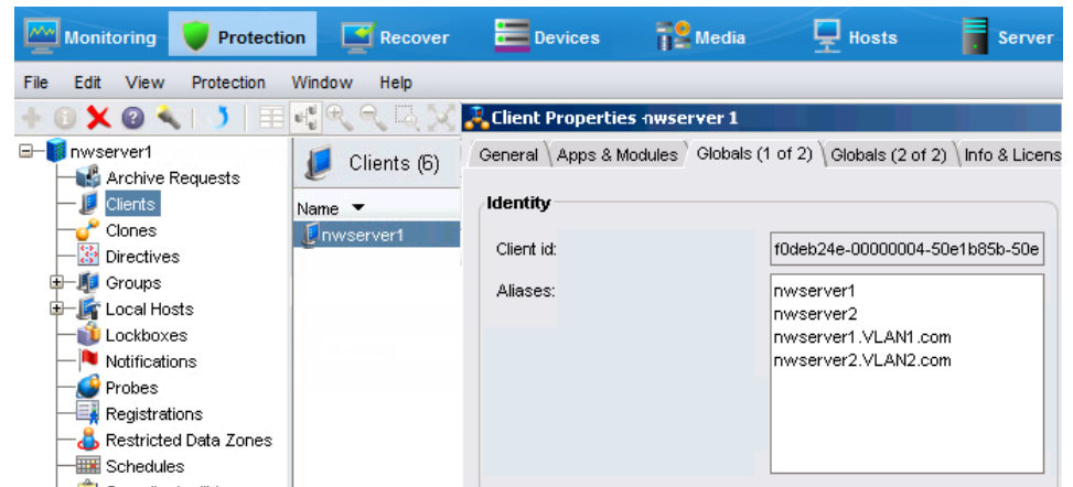
Figure 96 Configuring the Aliases attribute for NetWorker Server Client resource
