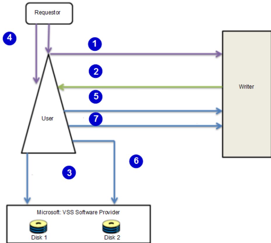
Figure 47 VSS backup process
