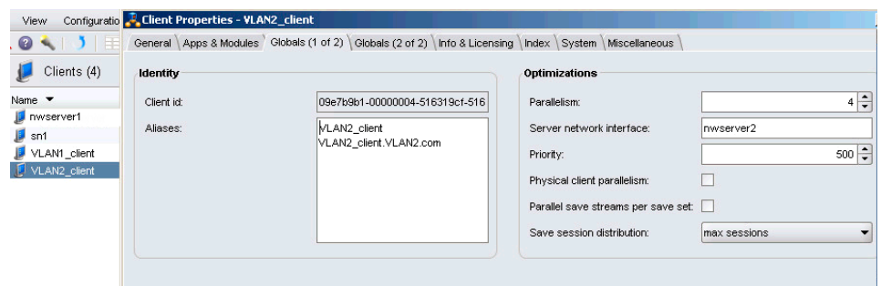
Figure 101 Aliases and Server network interface attributes for VLAN2 clients
