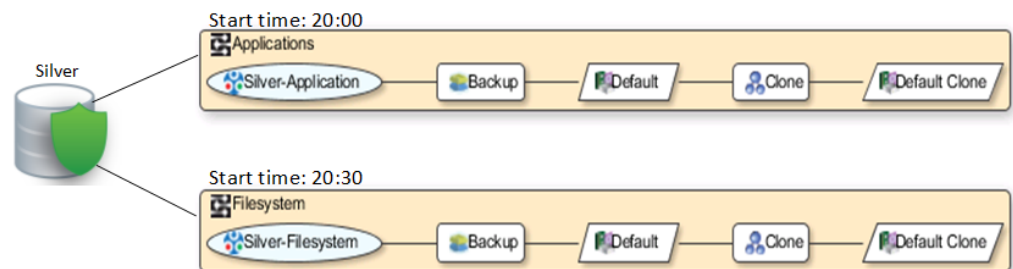
Figure 20 Silver policy configuration
