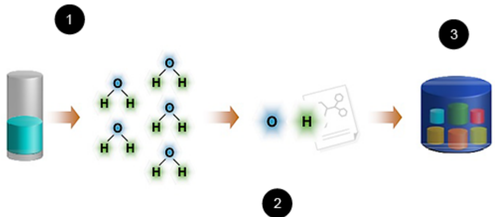
Figure 4 Data deduplication
