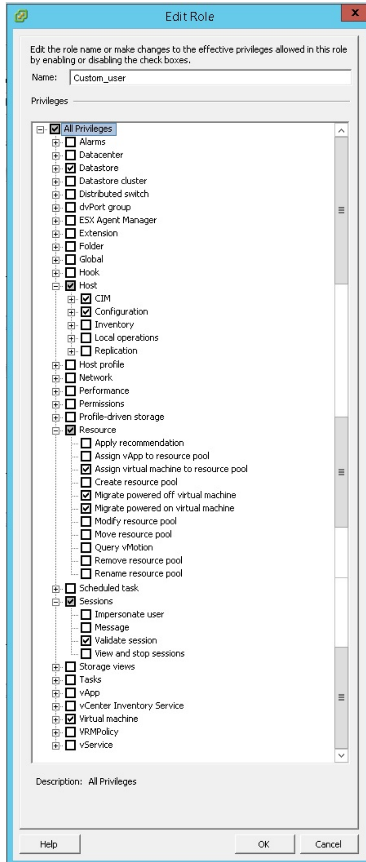
Figure 6 Privileges needed for VC roles for AppSync
