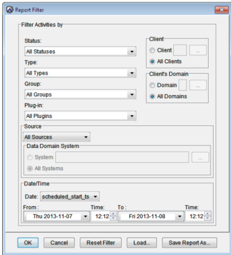
Figure 3 Report Filter dialog box
