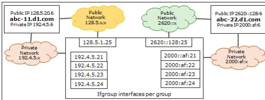
Figure 4 IFGROUP Support for IPv4 and IPv6 Addressing
