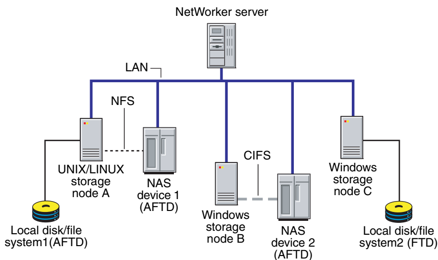
Figure 27 Sample NetWorker DiskBackup configuration
