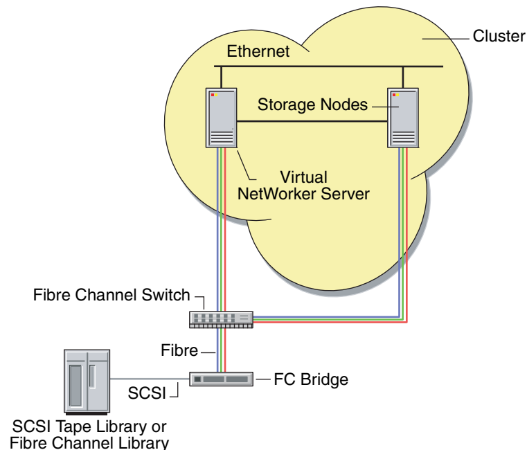
Figure 36 DDS enabled with robotics controlled in the cluster
