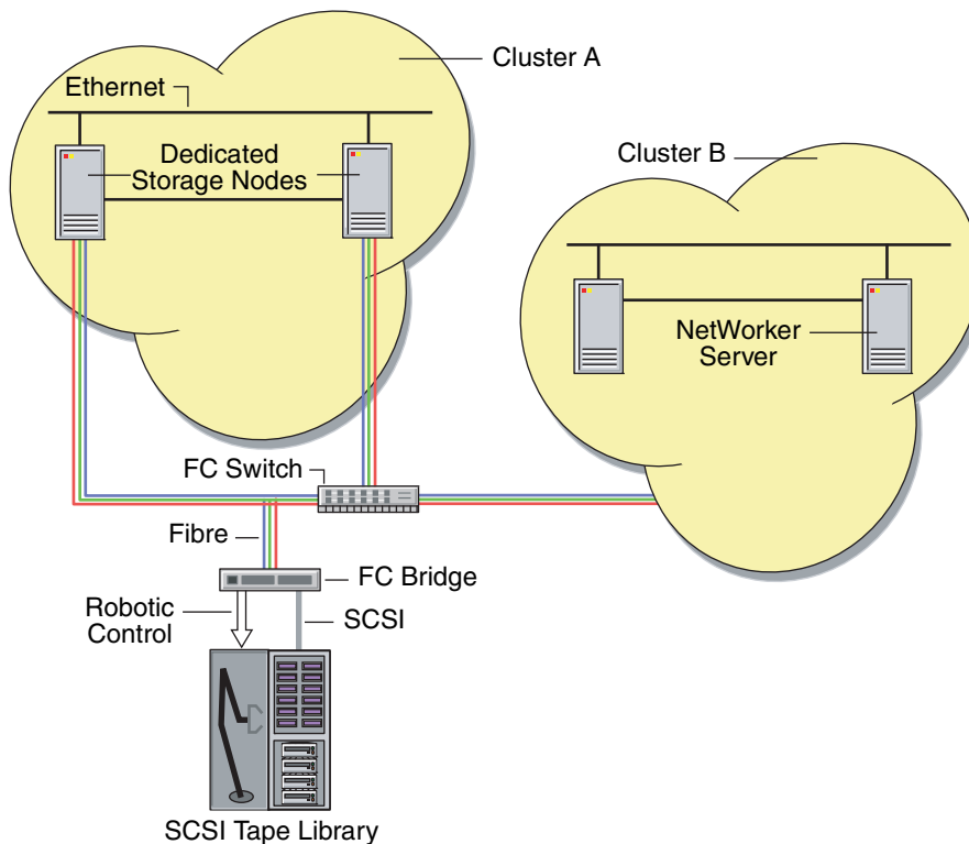
Figure 38 Robotics controlled between clusters
