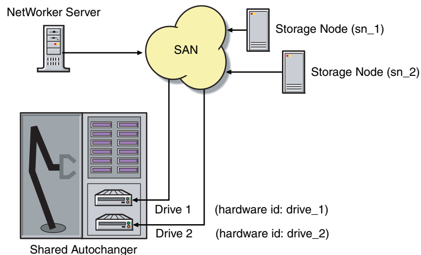
Figure 9 Dynamic Drive Sharing
