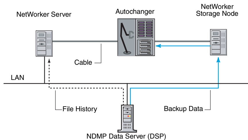
Figure 41 File history and backup data to NetWorker storage node
