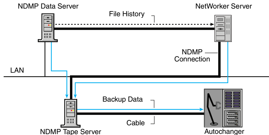
Figure 43 NDMP tape server
