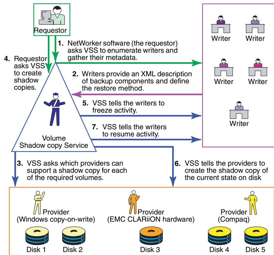
Figure 58 VSS backup process
