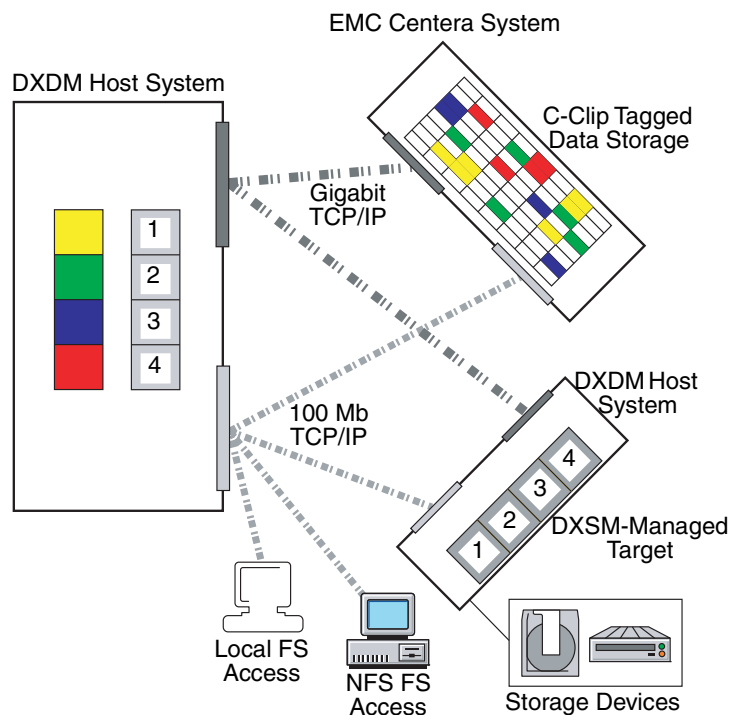
Figure 44 Prototypical DXDM installation
