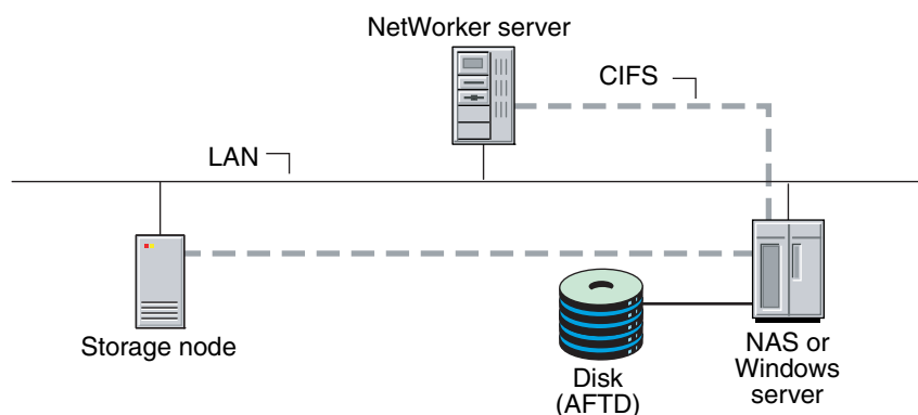
Figure 28 CIFS-mounted advanced file type device
