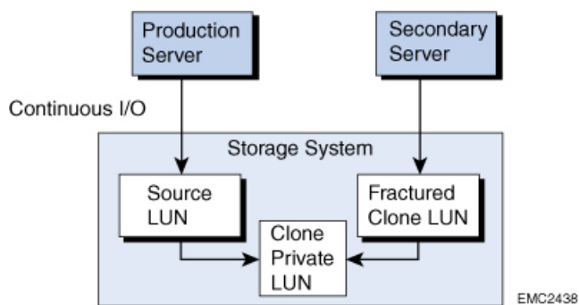
Figure 1. Clones example
