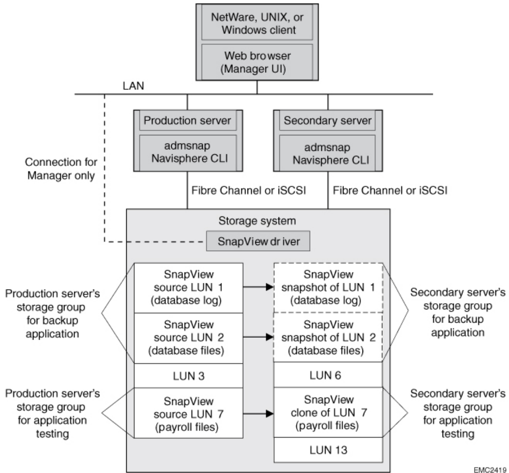
Figure 2. Sample SnapView environment with clones and snapshots
